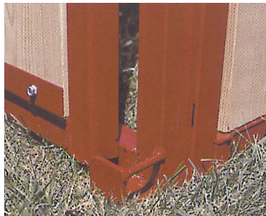
Standard roller-mounted sliding door on all stalls. Swing doors also available.
